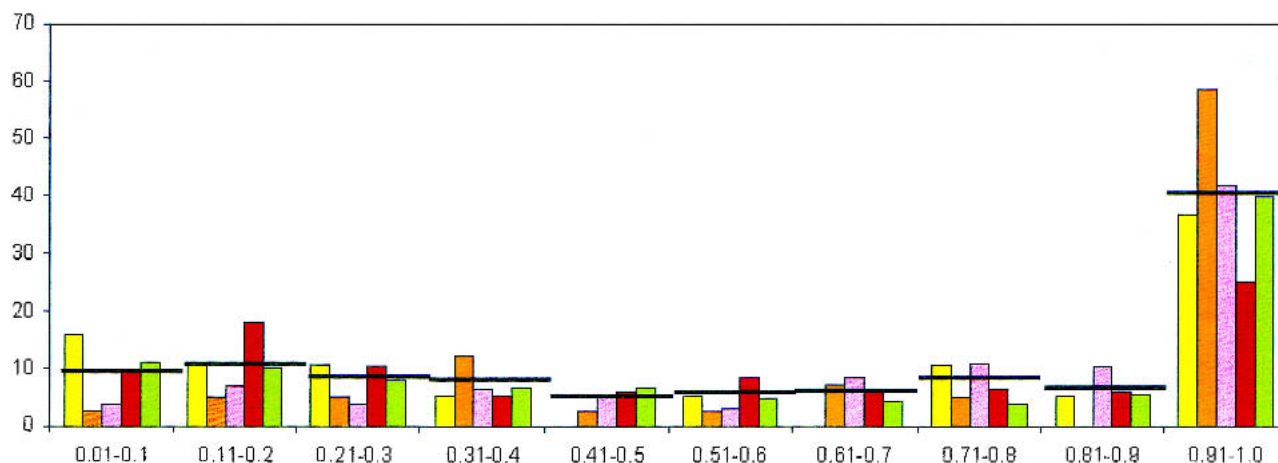
Figure 4 Distribution of lineage-specific clusters by Expansion Coefficient (EC). The X-axis shows ranges of EC values (see text) and the Y-axis shows the percentage of LSCs within each EC range. (Yellow) Schizosaccharomyces pombe ; (orange) Saccharomyces cerevisiae ; (pink) Drosophila melanogaster ; (red) Caenorhabditis elegans ; (green) Arabidopsis thaliana . In each class, the average value of the five species is indicated by a horizontal line.
