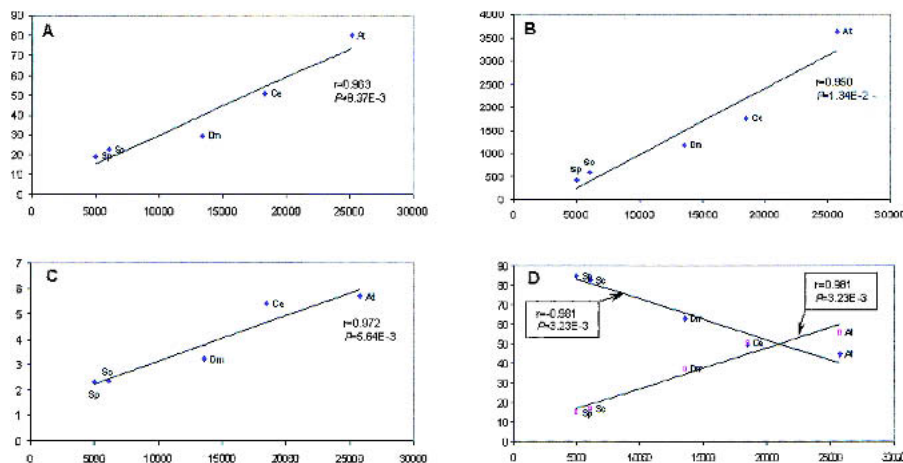
Figure 2 Linear correlation between the proteome size and parameters of eukaryotic lineage-specific expansion (LSE) in five eukaryotic species. Correlation coefficients ( r ) and significance levels ( P ) were determined using ordinary least square linear regression. (At) Arabidopsis thaliana ; (Ce) Caenorhabditis elegans ; (Dm) Drosophila melanogaster ; (Sc) Saccharomyces cerevisiae ; (Sp) Schizosaccharomyces pombe . (A) The proteome size (X-axis) is plotted against the percentage of the proteome made up of LSEs. (B) The proteome size (X-axis) is plotted against the number of lineage-specific clusters. (C) The proteome size (X-axis) is plotted against the mean number of proteins in lineage-specific clusters. (D) The proteome size (X-axis) is plotted against the percentage of duplication ( \blacklozenge ) and the percentage of n-plication ( n > 3 ) ( \square ) among the LSCs.
