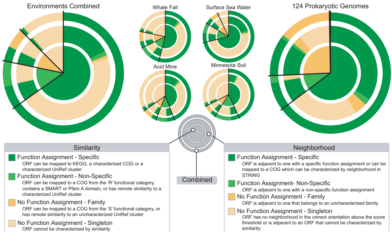
Fig. 2. Protein function prediction in genomes and metagenomes. Many proteins can be functionally characterized in both data sets. The degree of functional characterization for four metagenomic data sets is shown on the left and for 124 prokaryotic genomes on the right. The inner pie chart represents the level of functional characterization possible by using the homology-based approach. The middle ring shows the level of functional characterization possible by using neighborhood methods. The outer ring summarizes the combined level of characterization possible. Surprisingly, it implies that most metagenomic ORFs (83% of the data) can be functionally characterized, similar to the level possible in fully sequenced genomes.
